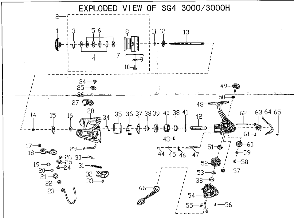
EXPLODED VIEW OF SG4 3000/3000H
